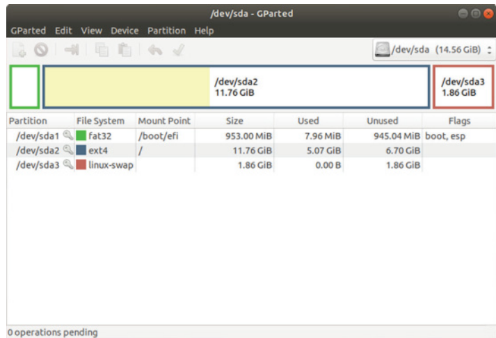
FIGURE 3.2 The GParted interface
